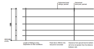
Type D estate railing Scale 1:20
